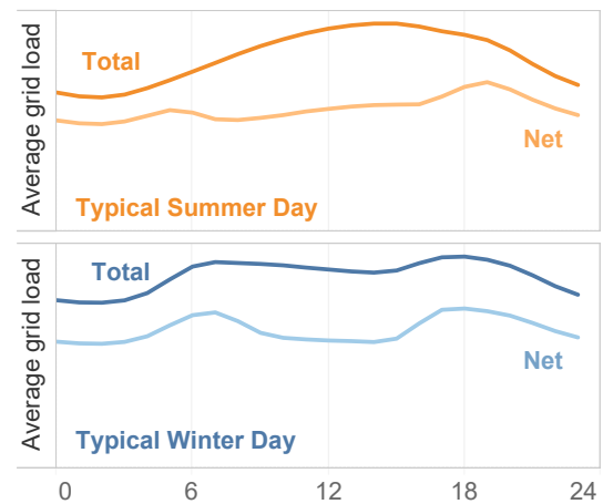
Midwest and Mid-Atlantic System Load Profile
