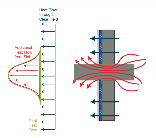
Figure 4: This diagram illustrates how lateral heat flow between assembly components allows additional heat flow through the thermal bridge that is not captured by U-factor.
