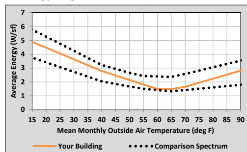
Energy Signature Comparison
