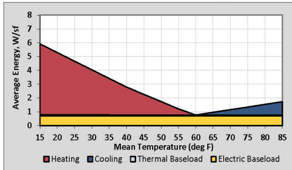
Consumption by End Use Energy Signature
